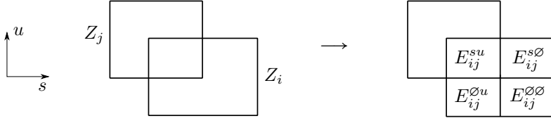
FIGURE 3. \mathcal{E}_{ij} = \{E_{ij}^{su}, E_{ij}^{s\emptyset}, E_{ij}^{\emptyset u}, E_{ij}^{\emptyset\emptyset}\} is a cover of Z_i by rectangles.
