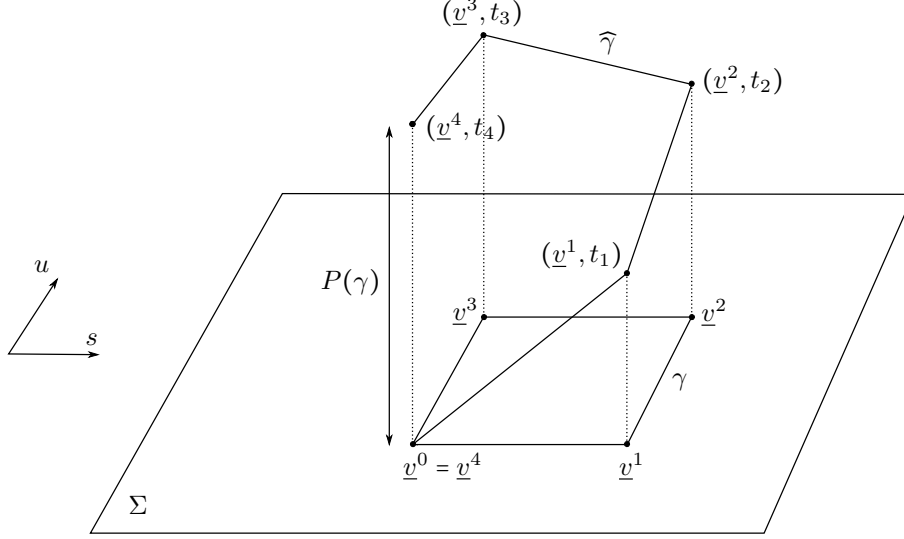
FIGURE 6. The holonomy group G : above \gamma is an su -loop forming a quadrilateral. The lift \widehat{\gamma} is not necessarily a loop.
