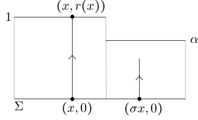
FIGURE 5. Totoki flow: a suspension over the shift on \{0, 1\}^{\mathbb{Z}} with uniform Bernoulli measure and piecewise constant roof function.
